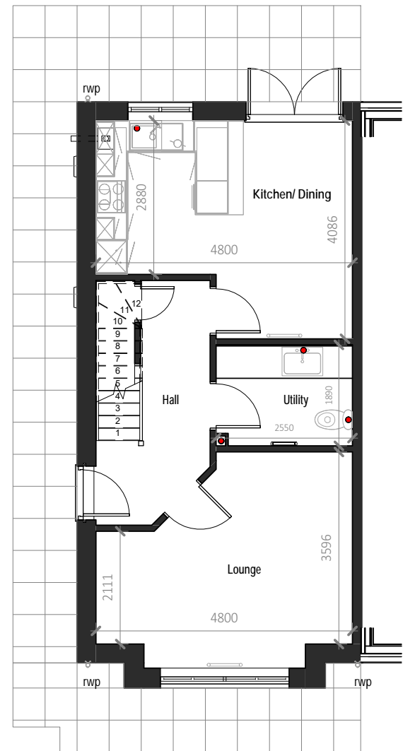
Ground Floor - Plan at A3 1 : 100 Plan at A1 1 : 50 Total internal area: 96m²
